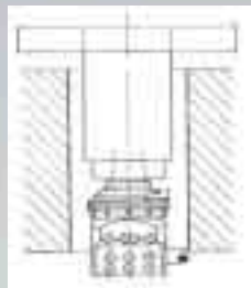
Because of the small construction of the facing and boring heads deep bores can be made. In this case the boring bit is fixed directly in the slide.
