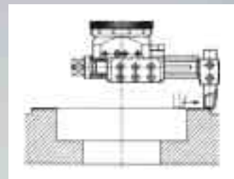
Facing of large \varnothing with long boring bar holder reinforced by rings and draw in screw.
